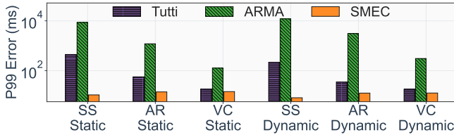
Figure 19: Accuracy of request start time estimation.
