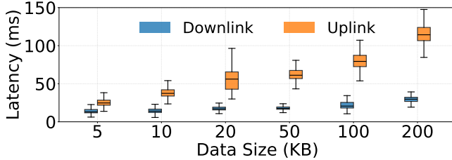
Figure 2: Network latency variability for uplink and downlink transmissions across different data sizes in City-1. Data size refers to request size for uplink and response size for downlink.
