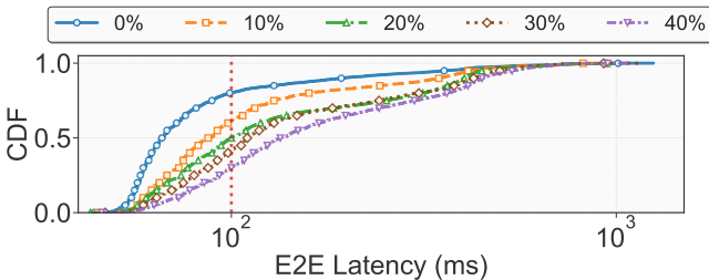
Figure 23: End-to-end latency for smart stadium under different levels of compute resource contention in City-2. The dotted red line indicates the SLO.
