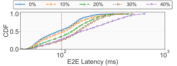
Figure 24: End-to-end latency for smart stadium under different levels of compute resource contention in City-3. The dotted red line indicates the SLO.
