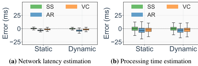
Figure 20: Accuracy of network and processing latency estimation.
