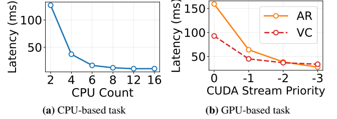
Figure 8: Relationship between compute resources allocation and process latency.
